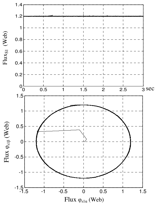
Fig.5.3.Electromagnetic flux behavior
