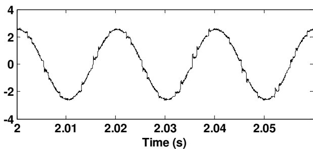
Fig.5.3.Electromagnetic flux behavior
