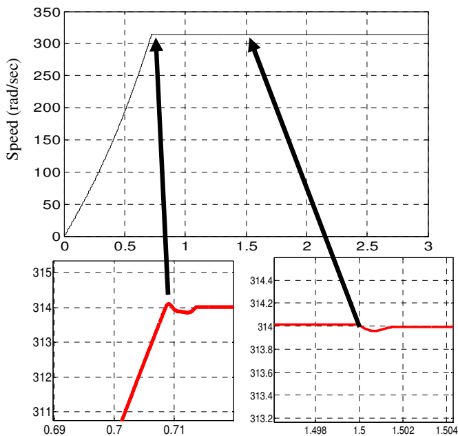
Fig.5. 1. PI Dynamic performance of FDTC on DSIM
