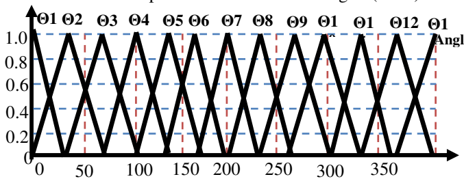
Fig.3.4.3.Membership functions for the position of the stator
