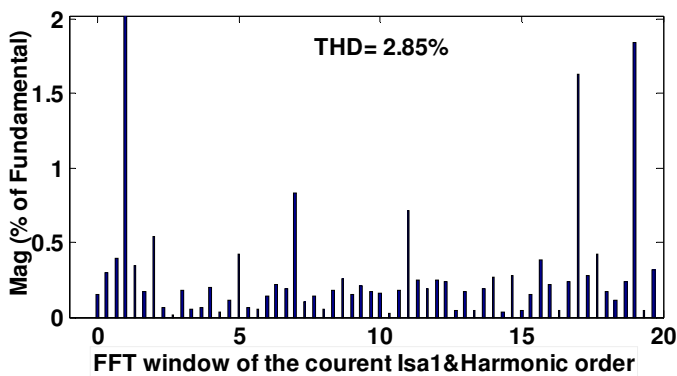
Fig 5.4. Harmonic order result of the stator current
