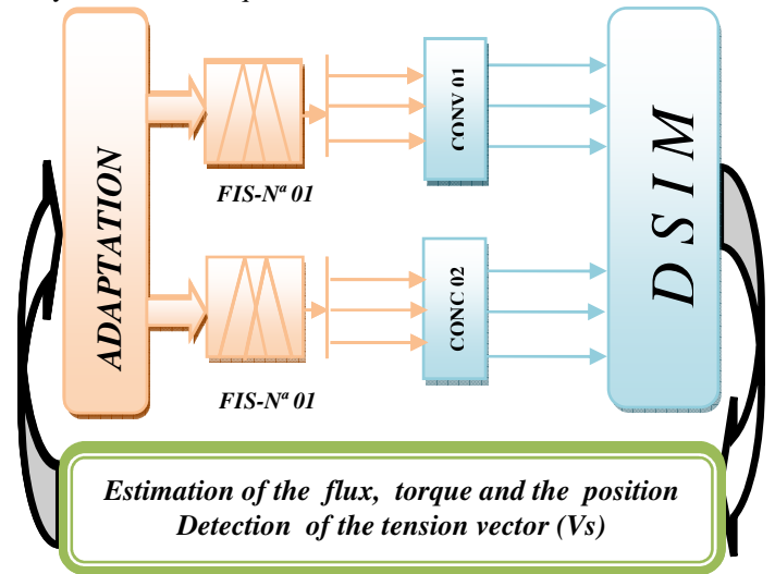
Fig.2.1. Block diagram of the fuzzy direct control of torque Application on the DSIM
