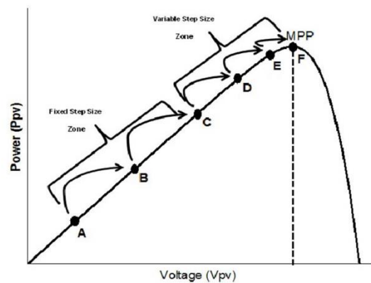
Fig. 4 A manner of tracking the MPP with variable step size increment.
