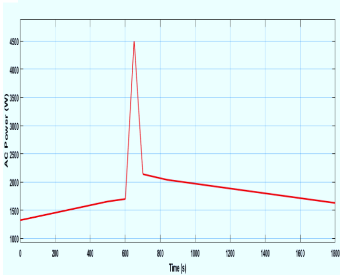
Fig 7 Four Solar Panels with DC-AC converter Efficiency 98%.
