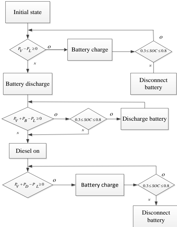
Fig7. Strategy of the control
