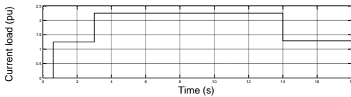
Figure 13 Load current profile
