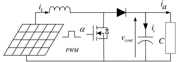
Fig6. Structure of the boost converter
