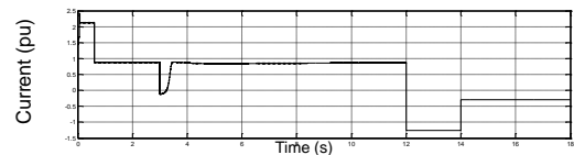
Figure 19. Battery Current
