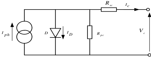
Fig4. Equivalent solar cell's electric circuit
