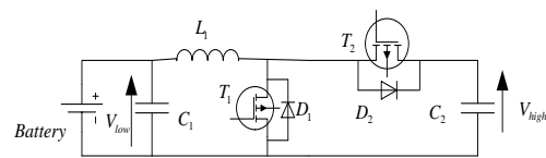
Fig11: Bi-directional DC/DC converter topology
