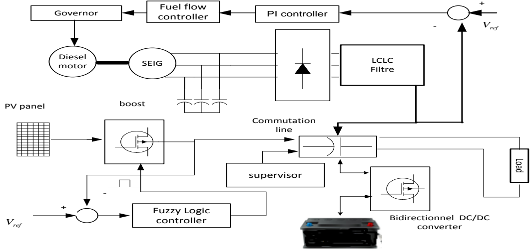
Fig1. The proposed Diesel-PV system
