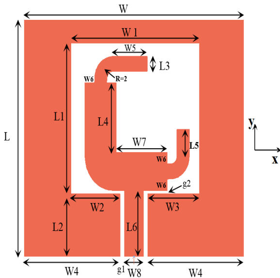
Fig. 1 Configuration of a proposed antenna.
