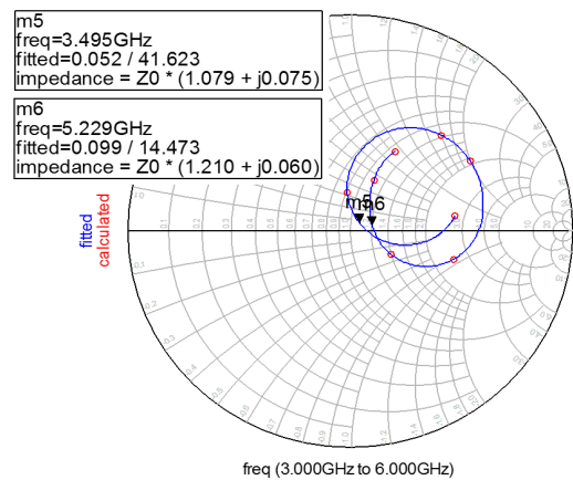
Fig. 3 Variation of impedance versus frequency.
