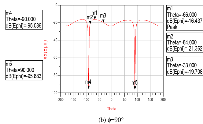
Fig. 8 Beamwidths of the antenna at 3.5 GHz with (a) \phi=0^\circ (b) \phi=90^\circ .
