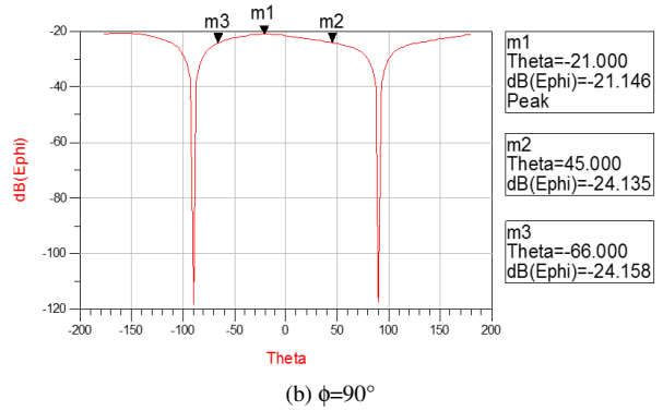
Fig. 13 Beamwidths of the antenna at 5.22 GHz with (a) \phi=0^\circ (b) \phi=90^\circ
