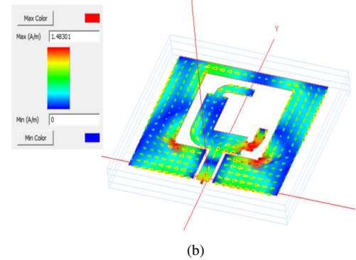
Fig. 14 Current distribution of the antenna at (a) 3.5 GHz (b) 5.22 GHz
