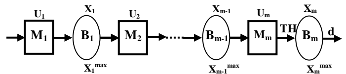
Fig.1 A serial line with m machines.
