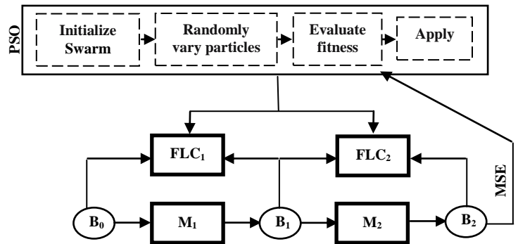
Fig.12 Distributed fuzzy PSO concept.
