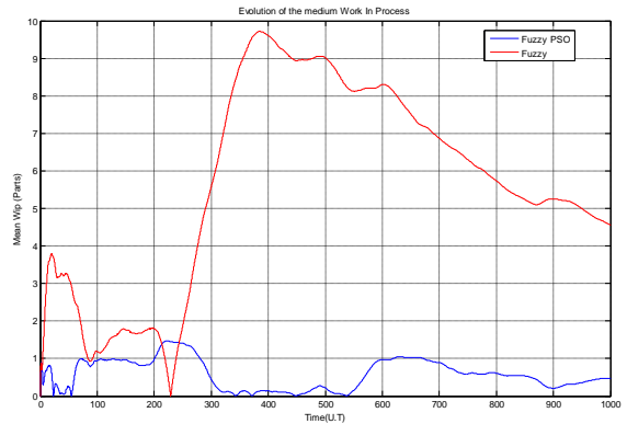
Fig.19 The medium WIP .
