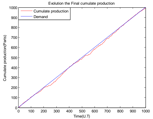
Fig.8 The cumulate production.
