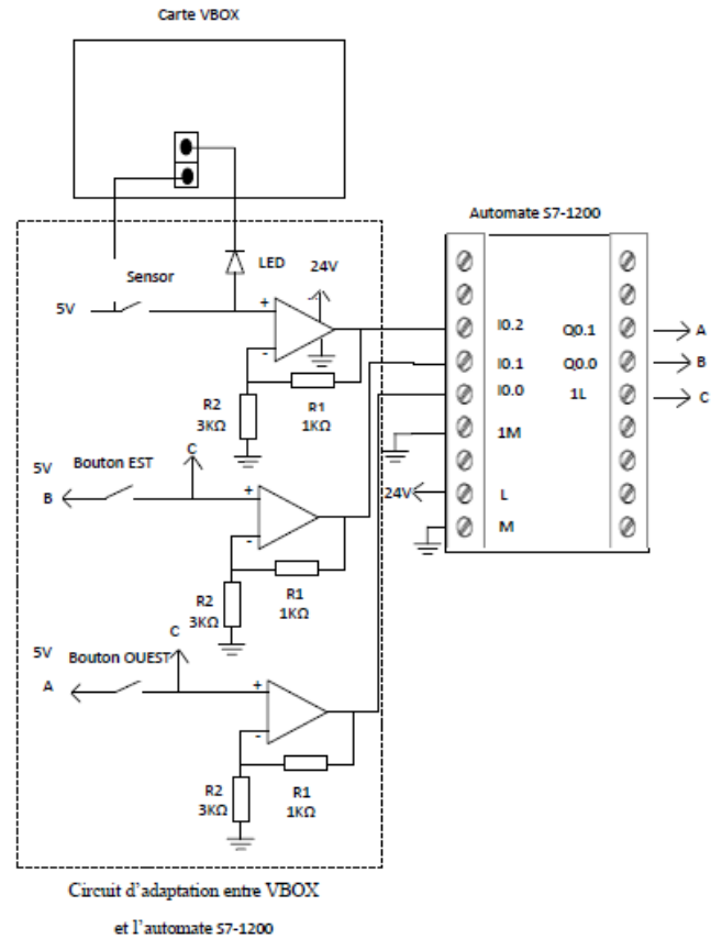
Fig 3. Adaptation of the programmable controller S7-1200 with VBOX
