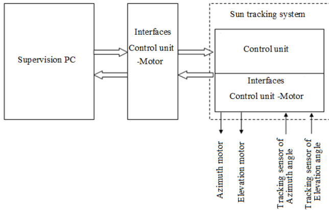
Fig. 1. Block diagram of sun tracking system
