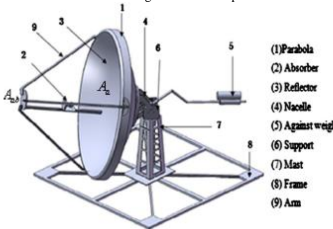
Fig 2. Structure of solar parabolic concentrator
