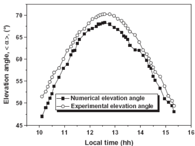
Fig. 5. Solar elevation angle.
