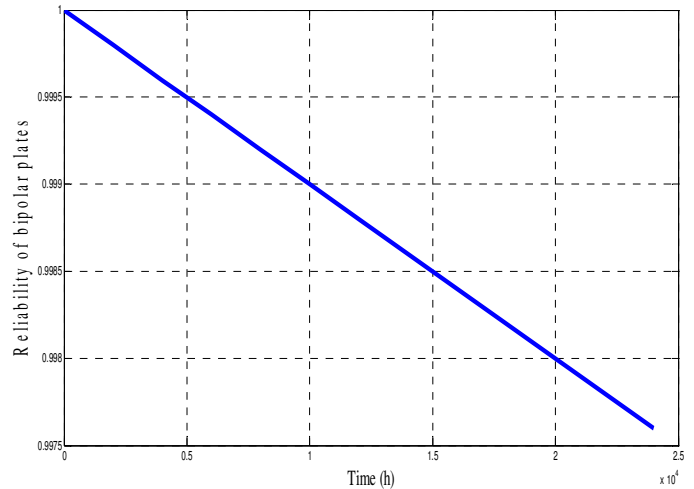
Fig. 5: Bipolar plates
