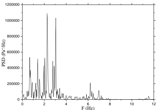
Fig.8 Exemple of bimodal spectrum ( J_1 = 0.566 m/s and J_g = 3.537 m/s)
