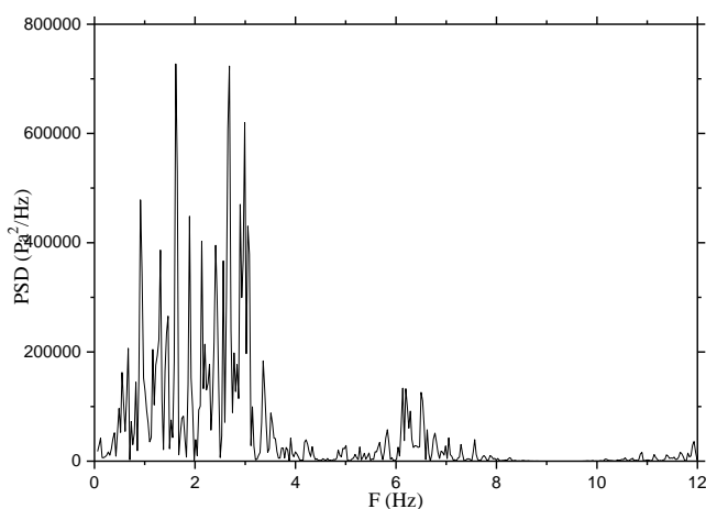
Fig.9 Exemple of trimodal spectrum ( J_1 = 0.707 m/s and J_g = 3.537 m/s)
