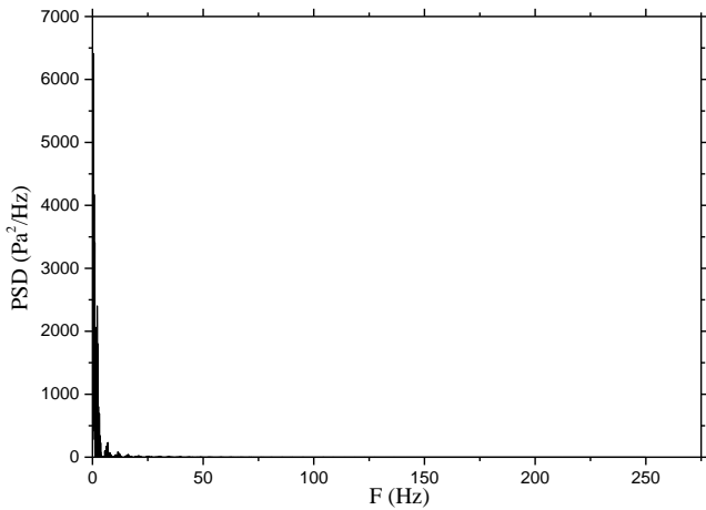
Fig.4 Example of frequency spectrum obtained by using the PSD ( J_1 = 0,141\text{m/s} and J_g = 1,179\text{ m/s} )
