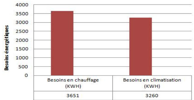
Fig.9. Comparison of Energy Requirements.
