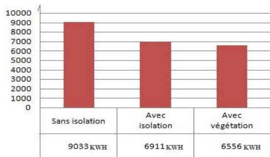
Fig. 11. Comparison of Energy Requirements / Yr.
