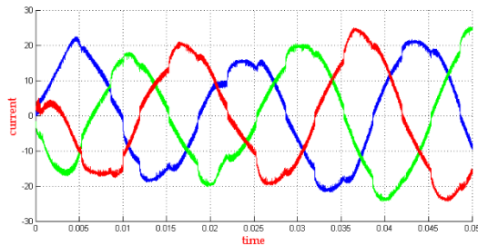
Fig.15 source current before filtering
