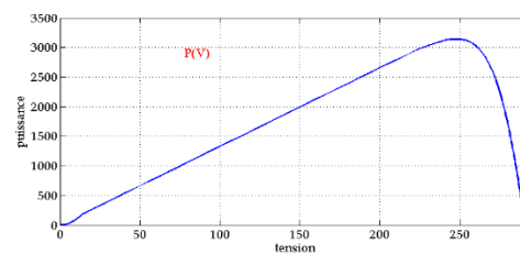
Fig.4 P-V curve
