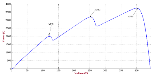
Fig.10 P-V curve under shaded conditions
