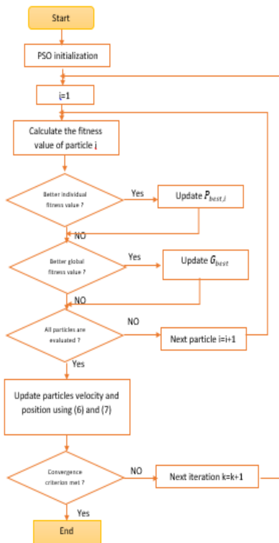
Fig.12 flow chart of standard PSO
