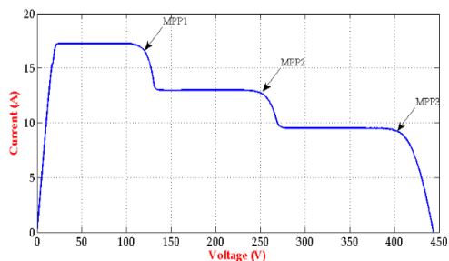
Fig.9 I-V under shaded conditions
