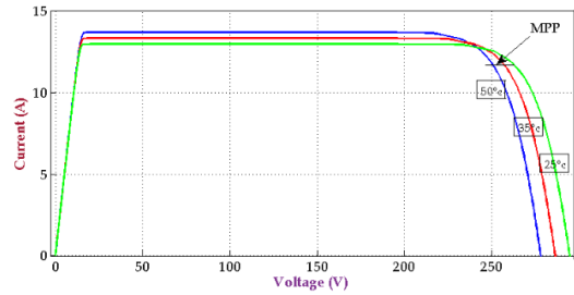
Fig.7 I-V curve with different values of temperature at 800w/m²
