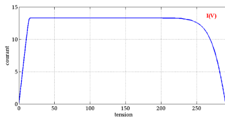
Fig.3 I-V curve
