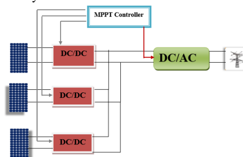
Fig.1 system configuration
