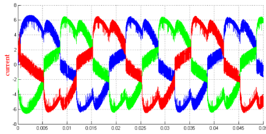
Fig.14 nonlinear load current
