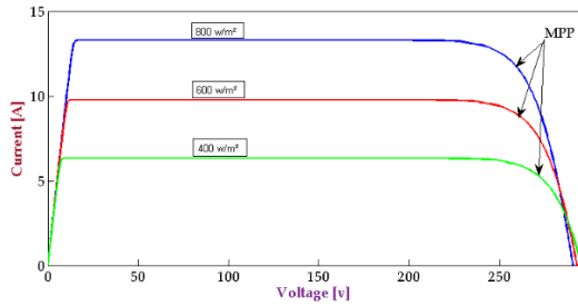
Fig.5 I-V curve for different values of radiation at 30°C
