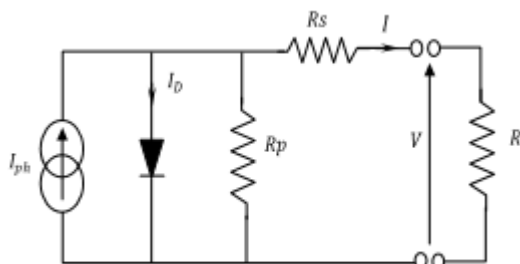
Fig.2 Solar Cell Equivalent Model
