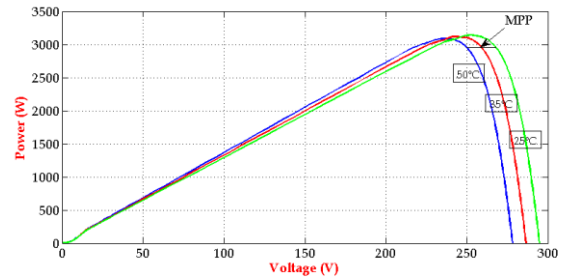
Fig.8 P-V curve for different values of temperature at 800w/m²
