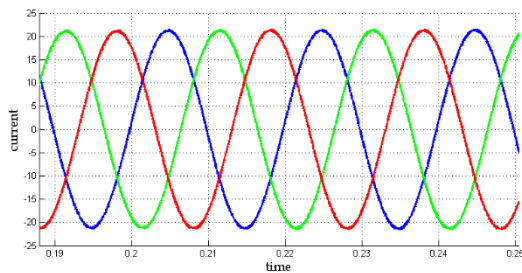
Fig.16 source current waveforms
