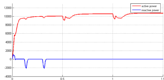
Fig.18 active and reactive power
